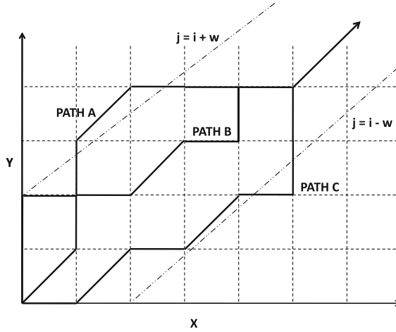
Figure 3.9: Illustration of warping paths
